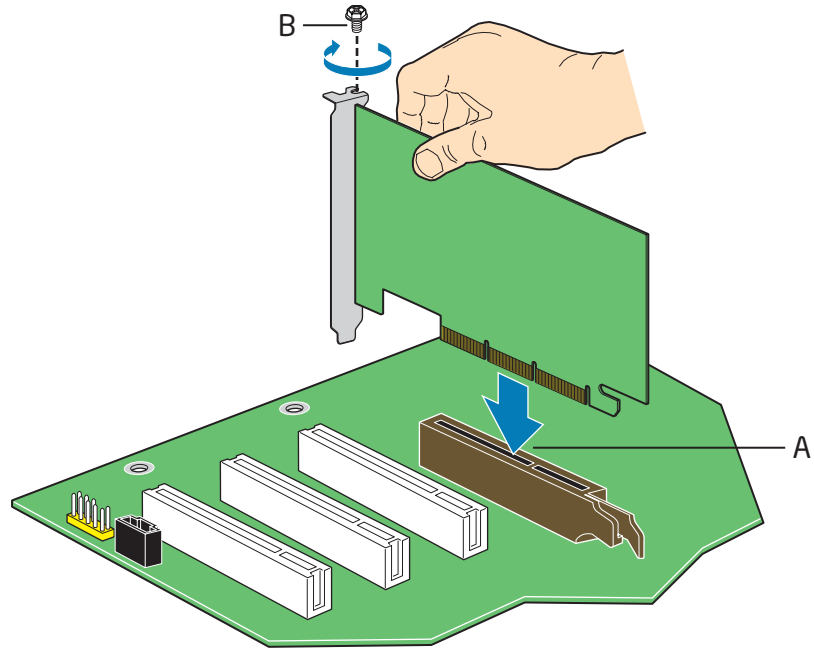
Figure 16. Installing an AGP Card
